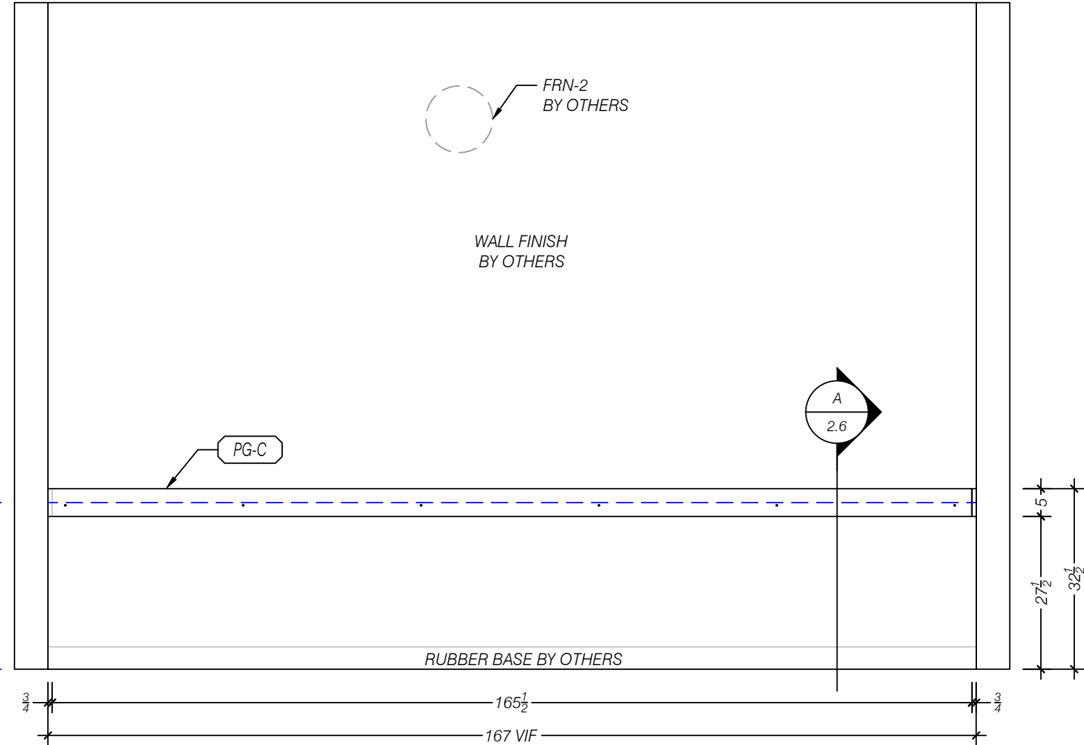
2 ELEVATION SOUTH - CONFERENCE 102 SCALE 1:24 (1/2"=1'-0") ARCH REF: 8/AE406
